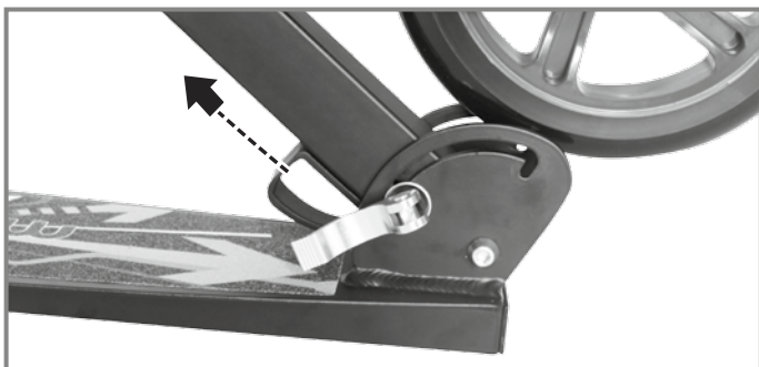
Pull the plastic handle upwards until the axle of the quick release locking system is released from the mount.
