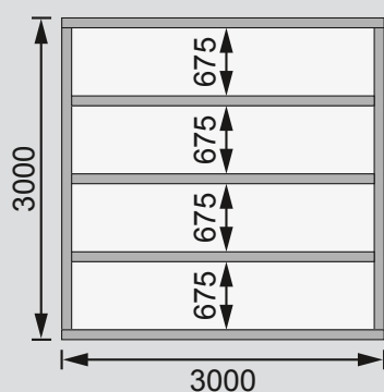
Fundamentplan (in mm)
