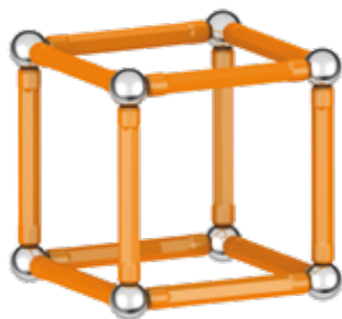
HEXAHEDRON (CUBE)
