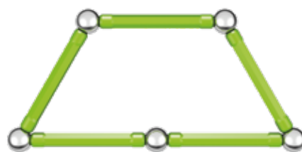
TRAPEZOID
