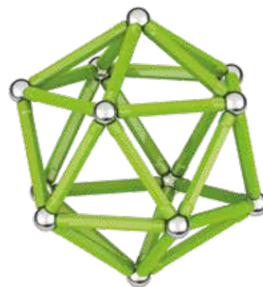
ICOSAHEDRON
