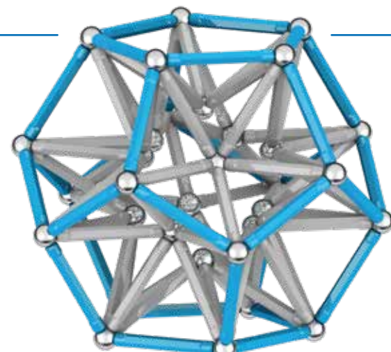
DODECAHEDRON
