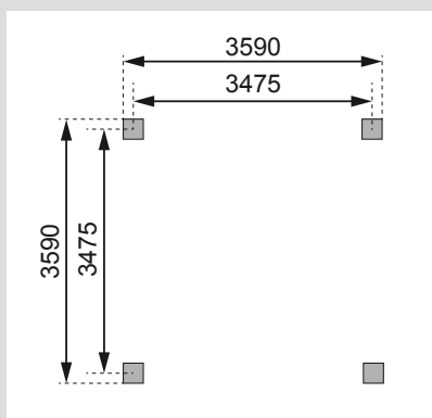
Fundamentplan Pfosten (in mm)
