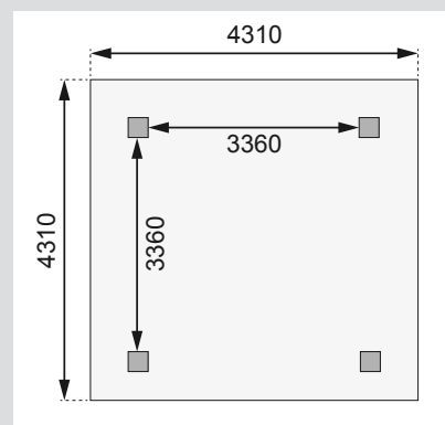
Dachstand / Pfostenanbstand (in mm)
