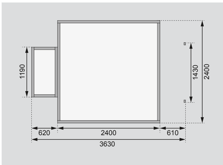
Fundamentplan (in mm)
